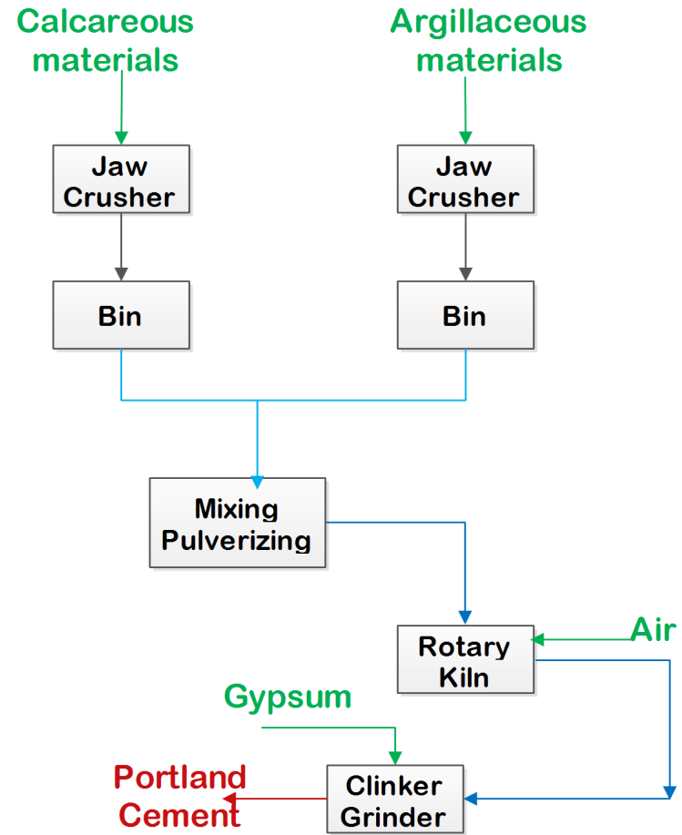
Figure: Manufacturing of Cement by Dry Process
